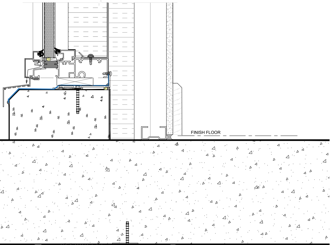
SILL DETAIL 3 @ Sandwich Panel on Curbs. SCALE: 1:3 ARCH. REF.:
