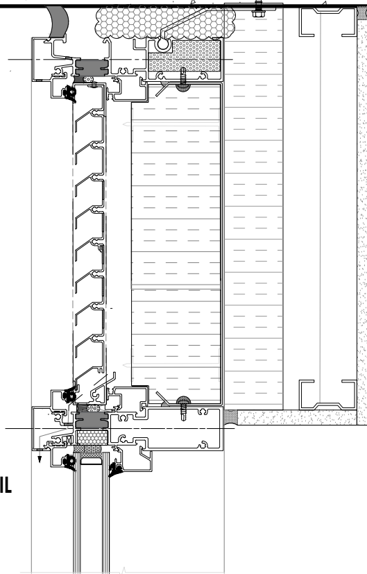
HEAD DETAIL 2 @ Louver SCALE: 1:3 ARCH. REF.: 6/A7-71
