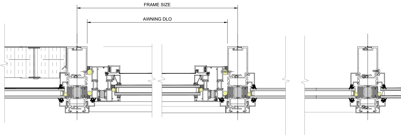
3 Awning Detail Vision/Vision ARCH. REF.:
